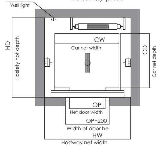
Hoistway plan
